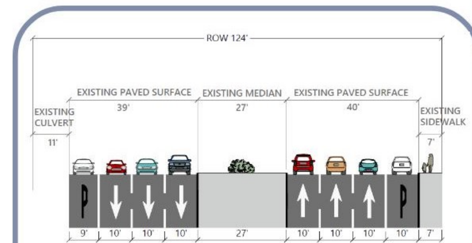
Cross-section at open channel
